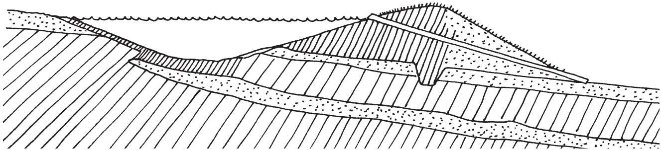
Figure 2. Precautions to Take During Construction of a Water Storage Structure to Prevent Seepage
