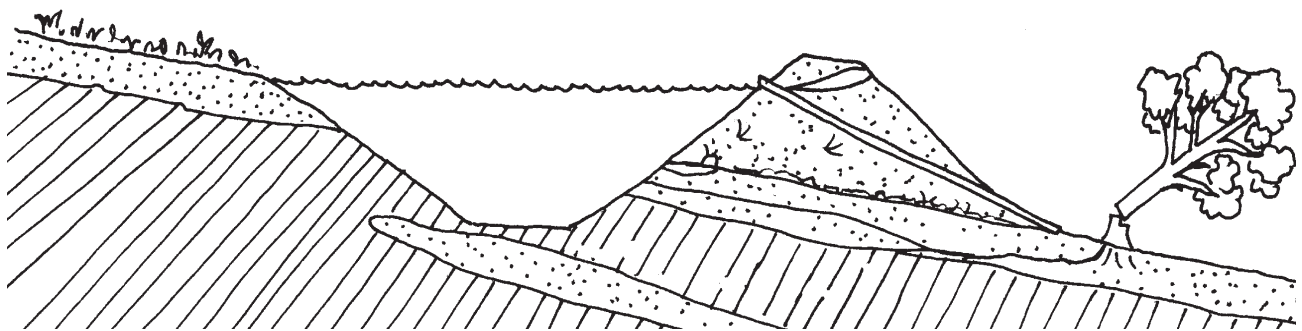
Figure 1. Situations in Which Seepage May Occur from a Water Storage Structure
